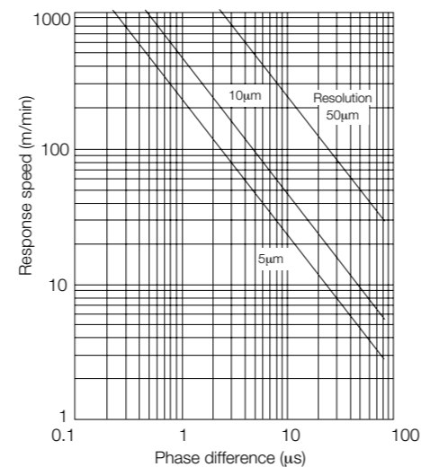
Response speed of PL60
